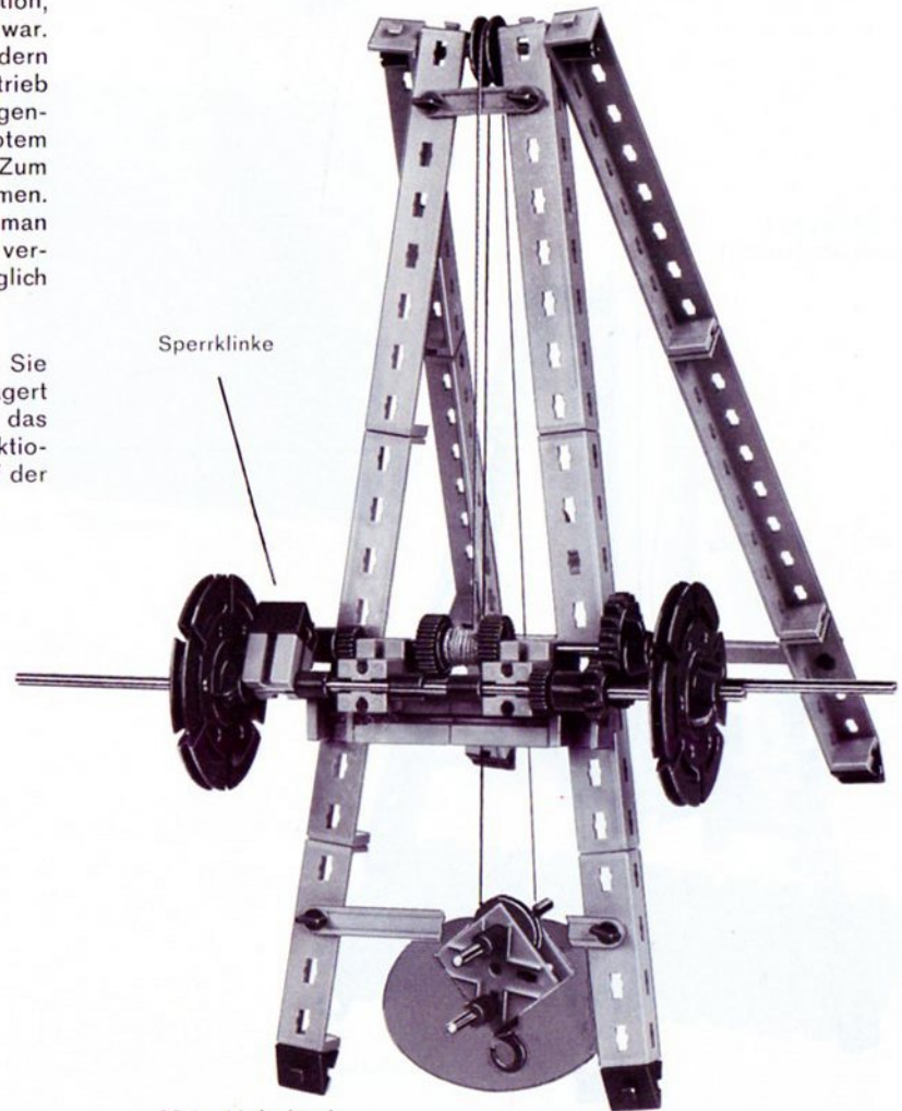
20.1 Hebebock
